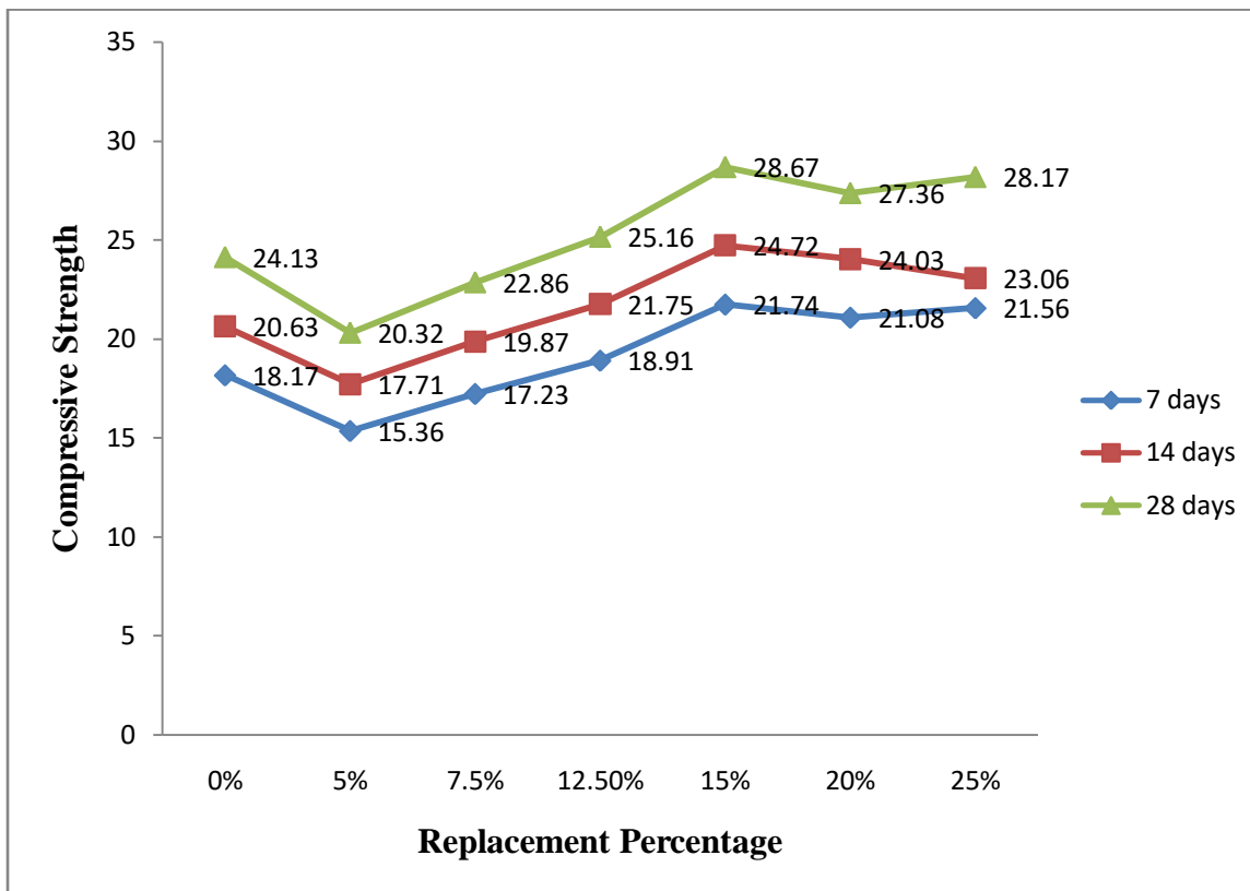
Graph: Compressive Strength in N/mm^2 at various age (Days) (Stage-1)
