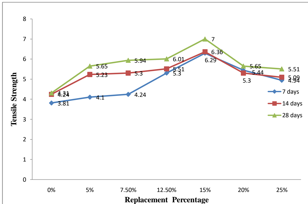
Graph: Split Tensile Strength in N/mm 2 at various age (Days) (Stage-1)
