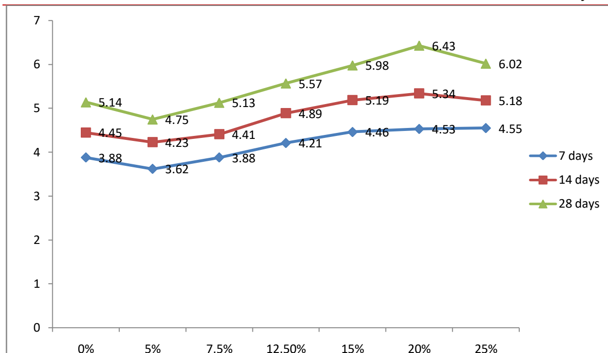
Graph: Flexural Strength in N/mm 2 at various age (Days)
