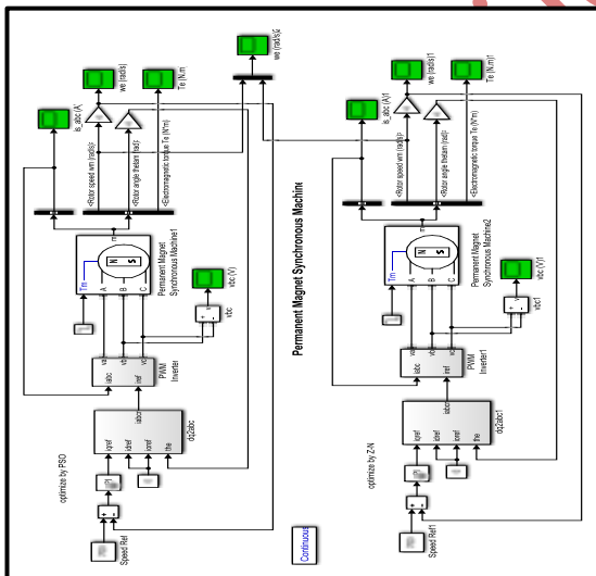
Fig 3 Comparative MATLAB simulation model of PMSM motor
