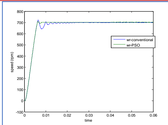
Fig.6 Comparative response of speed of PMSM motor concerning the time
