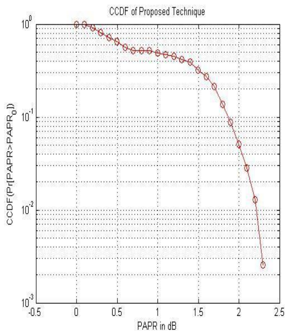
Fig.7 CCDF Proposed Technique
