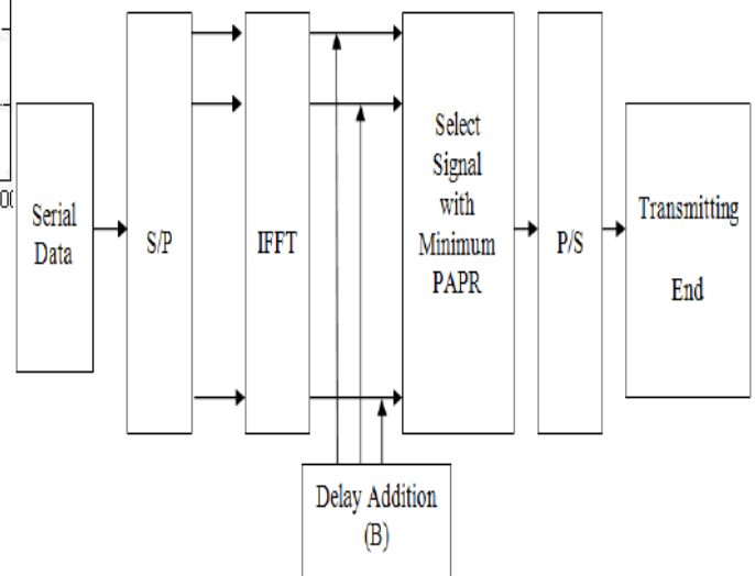
Fig.3 Block Diagram of SLM Technique
