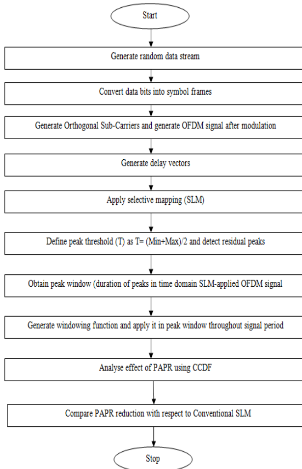
Fig.4 Flowchart of Proposed Technique
