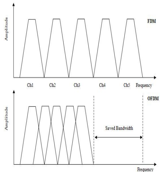
Fig.1 Comparative Analysis of FDM and OFDM.
