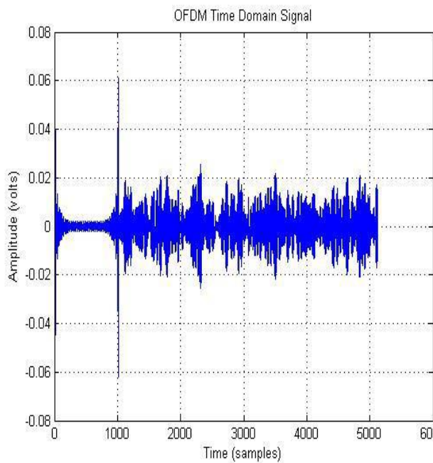
Fig.2 OFDM Time Domain Signal
