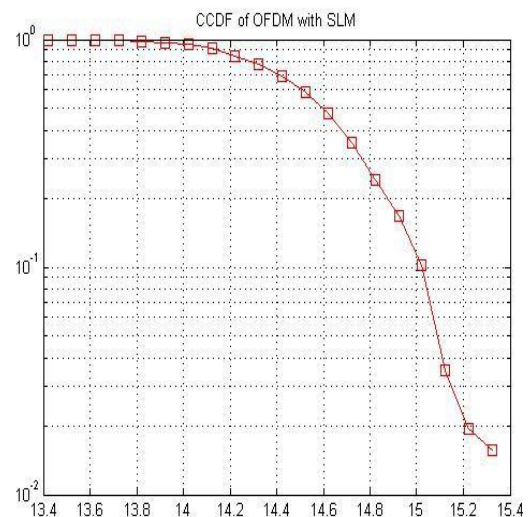
Fig.6 CCDF of Conventional SLM
