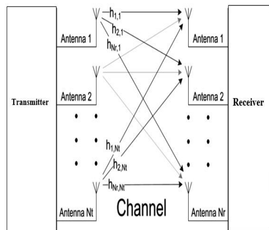
Fig.3. Conceptual model of a MIMO system
