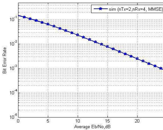
Fig. 8. BER Analysis for 2X4 MIMO with MMSE
