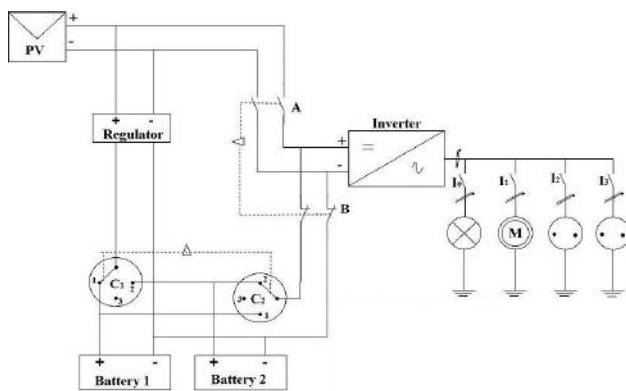
Figure 1. Flow chart of the photovoltaic system.
