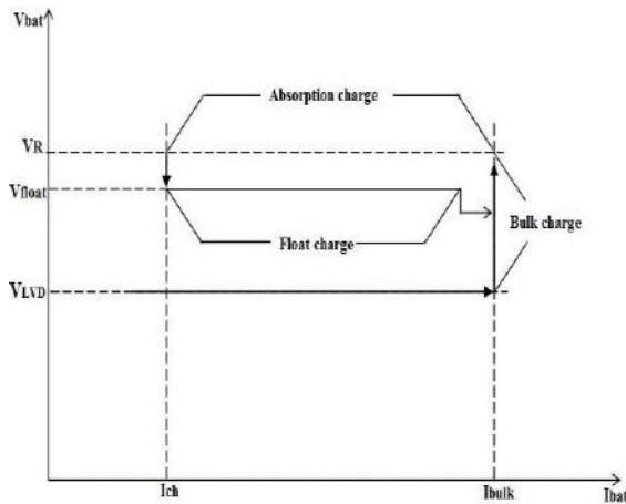
Figure 2: Different states of battery charge [23].
