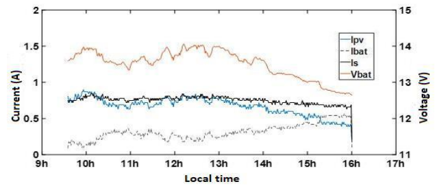
Figure 12: Currents Ibat, Ipv, Is and Vbat in day mode, recorded on 15 November 2023 in Ngaoundéré
