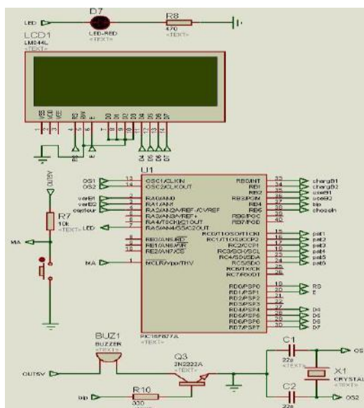
Figure 8: Control circuit of the facility.
