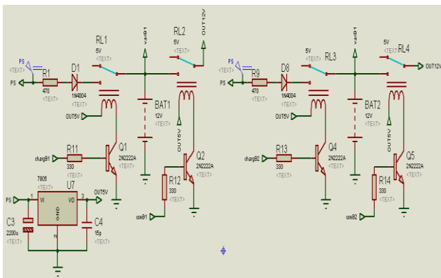
Figure 5: Electronic diagram of the supply circuit
