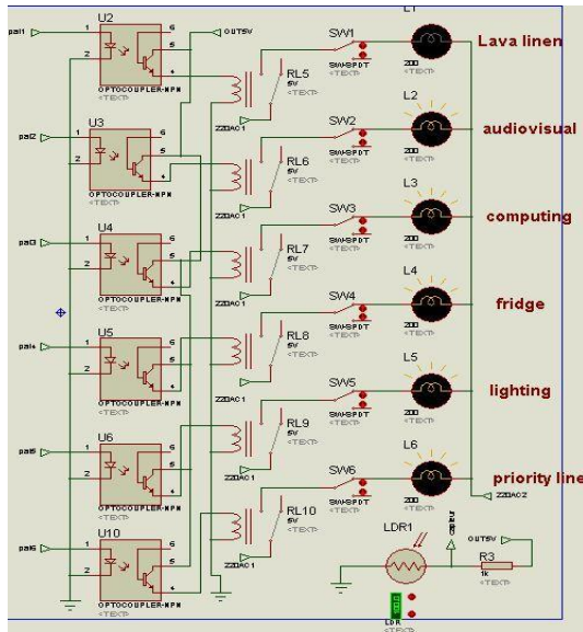
Figure 7: Circuit of the switches.
