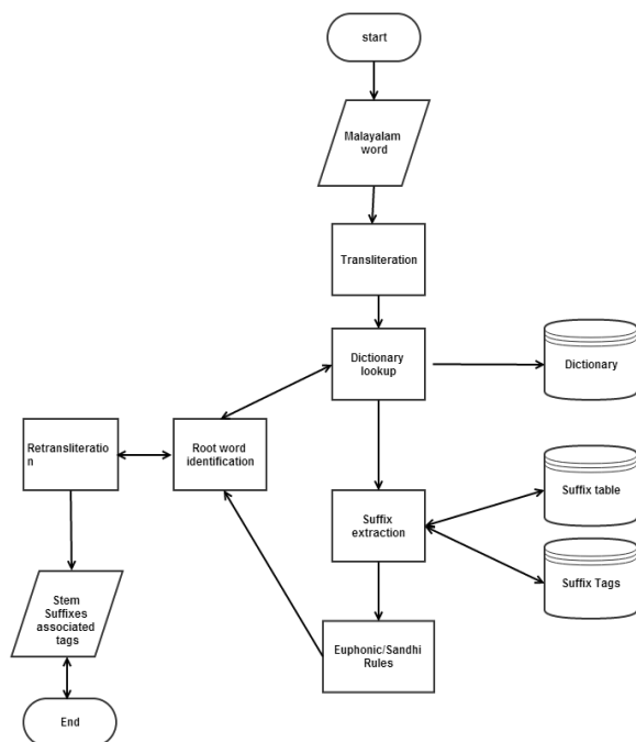
Figure 1. showing the data flow diagram of morphological analyzer for Malayalam word and verb
