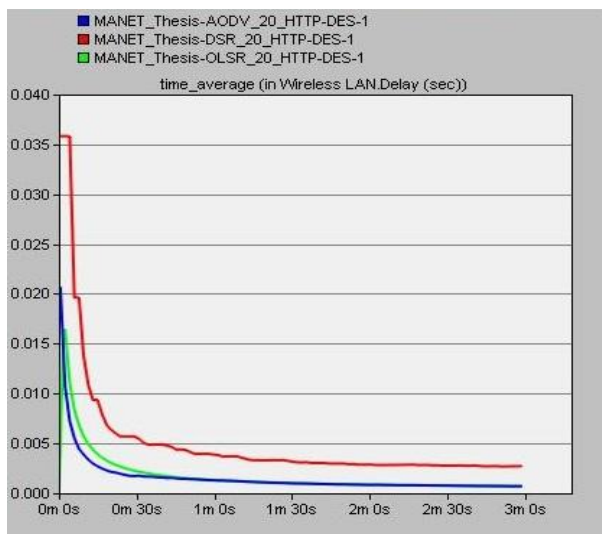
Fig 1: Delay comparison in three routing protocols for 20 nodes
