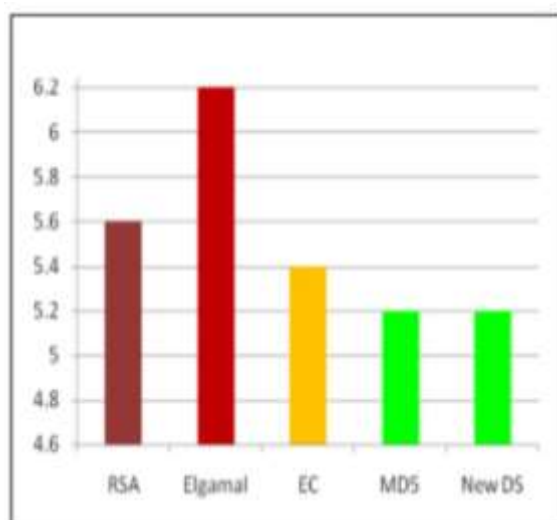
Fig 2: Result Analysis
