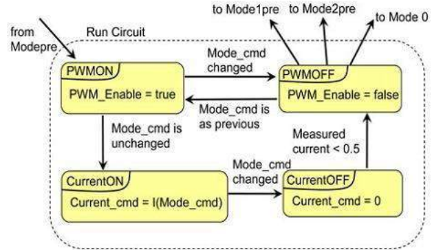
Figure 13. Control topology inside Run Circuit.
