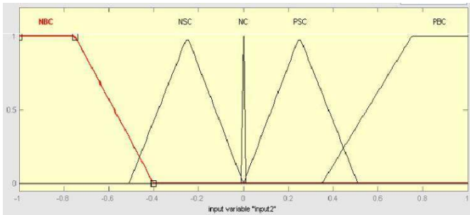
Figure 14.b. Membership function of change of error
