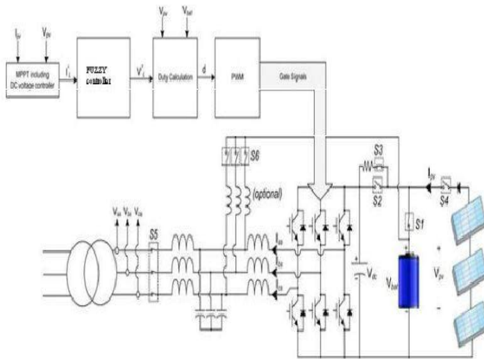
Figure 7. Overall control block diagram of the RSC in the dc/dc operation
