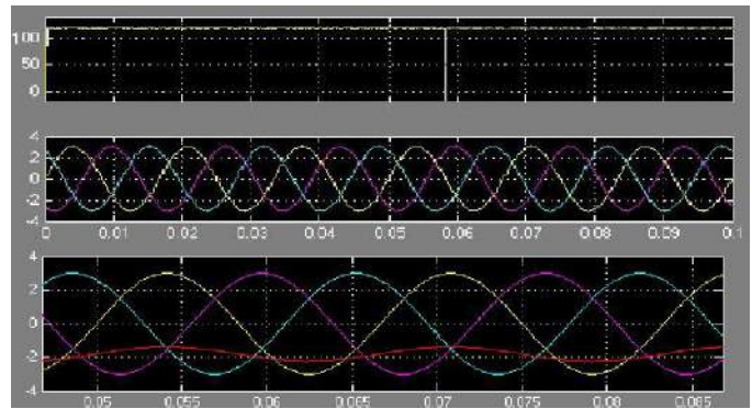
Figure17. Steady-state performance of dc /ac control in Mode 4
