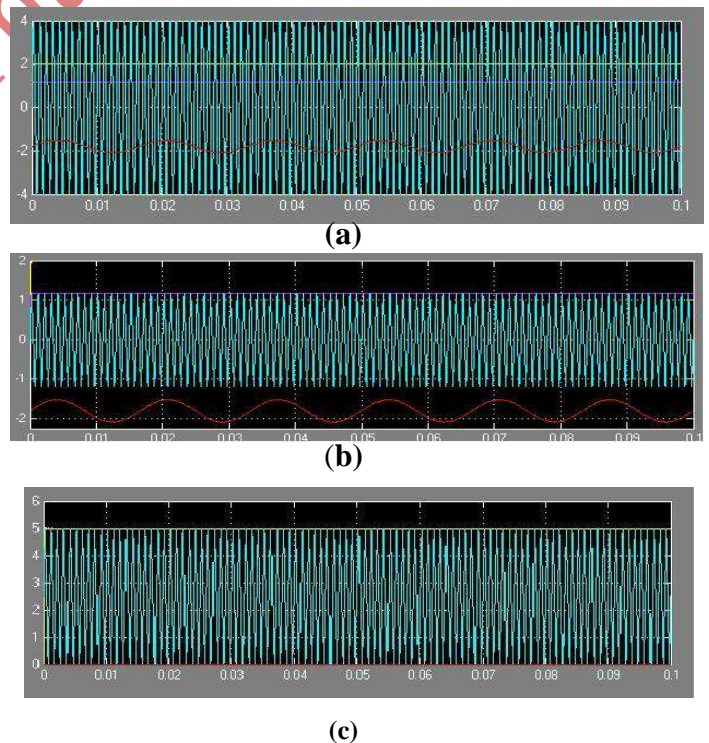
Figure 18. Steady-state performance of the RSC with single-phase operation in the dc/dc mode (Mode2). (a) When switches unused are not turned OFF. (b) When switches unused are turned OFF. (c) When three single-phase inductors are used
