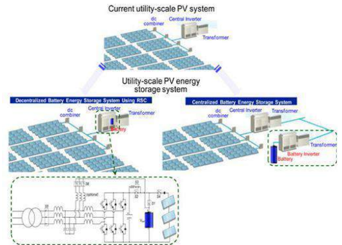
Figure 4. Utility-scale PV-energy storage systems with the RSC and the current State-of-the-art solution.
