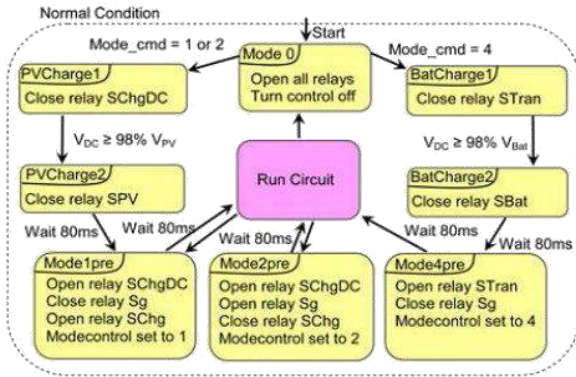
Figure 12. States inside Normal Condition.
