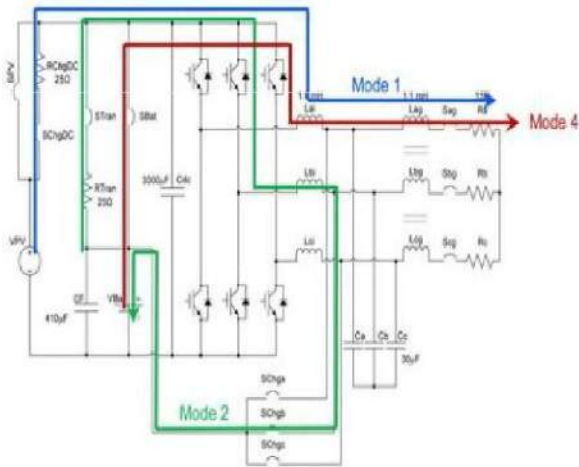
Figure15. Different operation modes tested in the lab.
