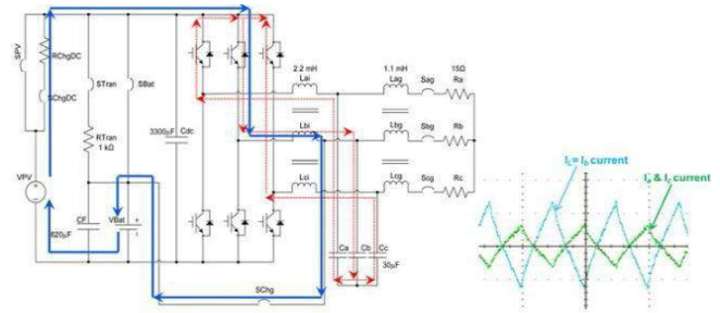
Figure8. Circulating current path if one phase is used for the dc/dc operation of the RSC with a coupled three-phase inductor
