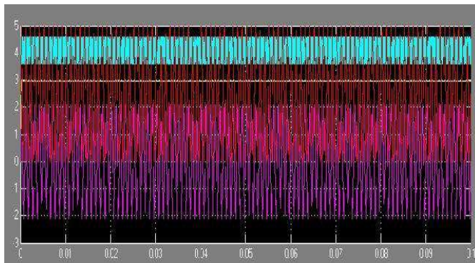
Figure 19. Steady-state capacitor and battery current for single phase operation using three single-phase inductors in the dc/dc operation.
