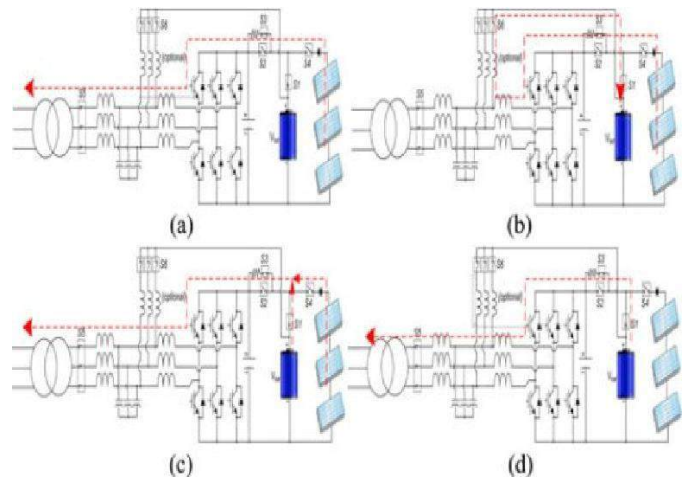
Figure3. All operation modes of the RSC. (a) Mode 1—PV to grid (b) Mode 2—PV to battery (c) Mode 3—PV/battery to grid (d) Mode 4—battery to grid
