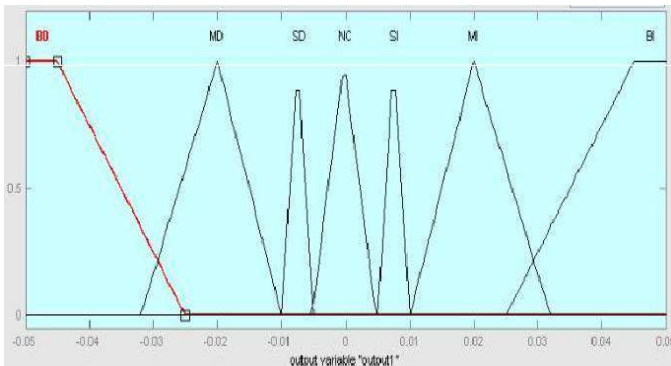
Figure 14.c. Membership function of output
