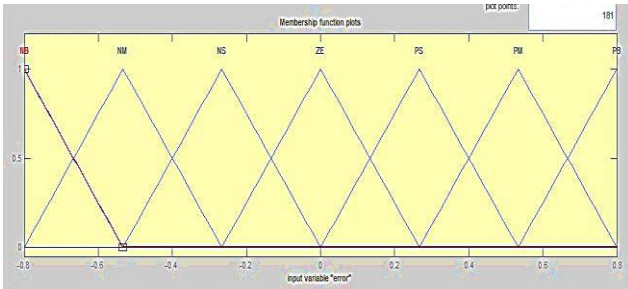
Fig.5.Membership function of error
