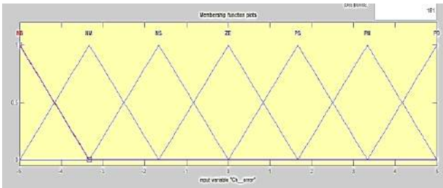
Fig.6.Membership function of change in error
