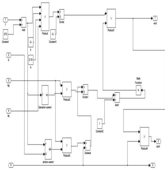
Fig.11. Simulink model of a PV array
