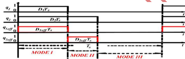
Fig.4.Switching diagram of the MI Cuk dc-dc converter[14].
