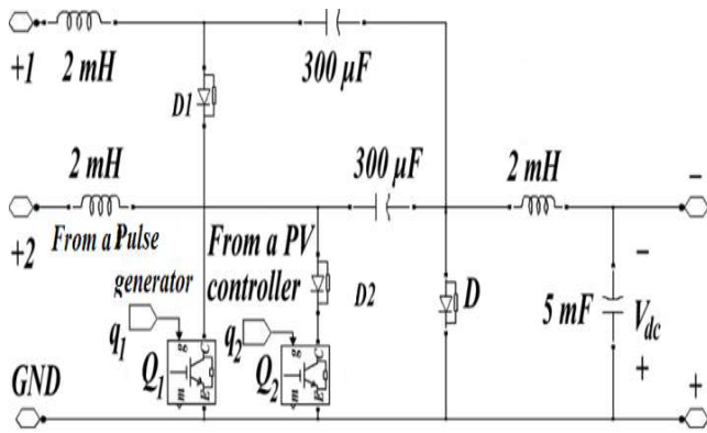
Fig.10. Schematic of the MI Cuk converter.
