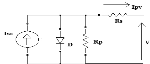
Fig.2.Single diode model of solar cell with Rs and Rf
