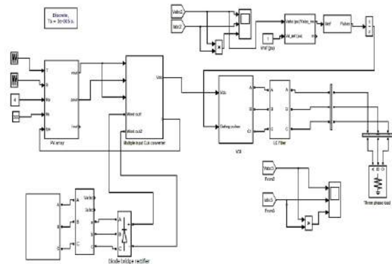
Fig.9. Overall simulation diagram of the proposed system Fig.9 shows the overall simulation diagram of 30-KW Wind/solar hybrid power system. The wind turbine is modeled using the equations (4) and (5).The specifications of the wind turbine and PMSG are specified elaborately in Tables I and II respectively. Fig.8 explains the controller which implements the incremental conductance control which is used to track the MPPs of solar energy as discussed in section VI-B. The MI cuk converter is modeled with built in components of MATLAB simulink /simpower systems.
