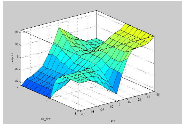
Fig.8. Rule surface of FLC
