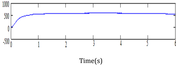
Fig.17 Multiple input cuk converter output voltage
