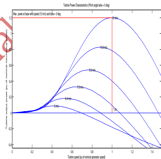
Fig. 13 Wind turbine output characteristics
