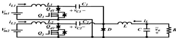
Fig.3.MI cuk DC-DC converter [10]
