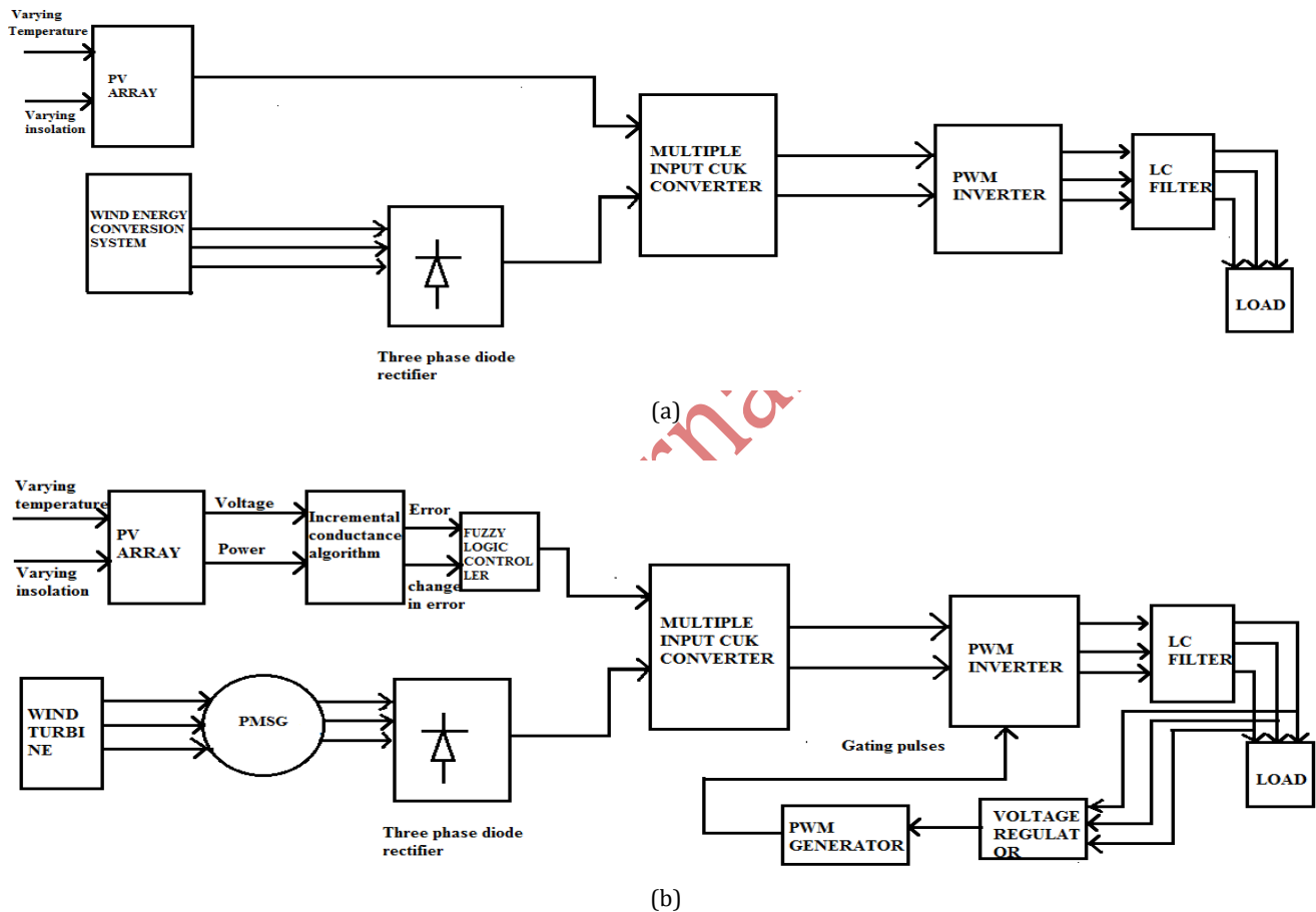
Fig.1.a) Power circuit of the proposed system
