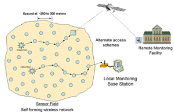
Figure 3: Incursion detection
