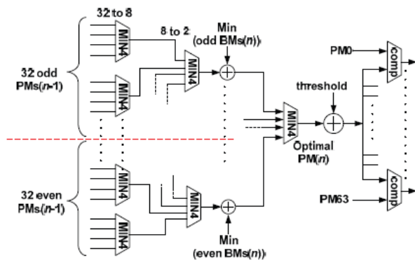
Figure 8. Implementation of 1-step pre-computation T-algorithm.
