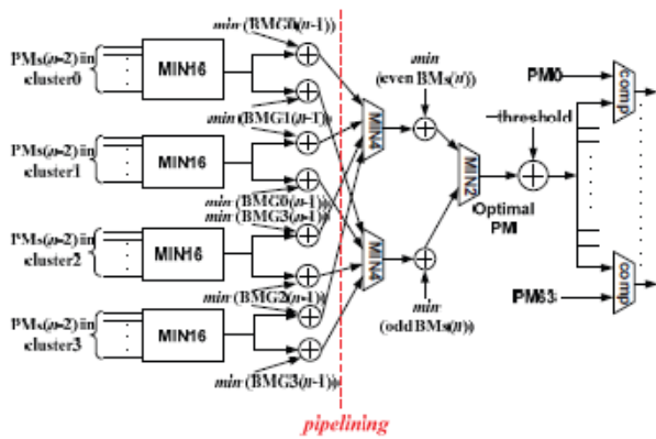
Figure 9. Implementation of 2-step pre-computation T-algorithm
