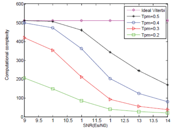
Figure 4. Computational complexity of T-algorithm
