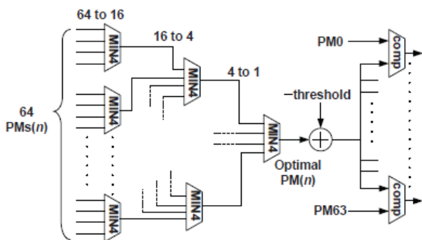
Figure 6. The implementation of PPAU for conventional T-algorithm.
