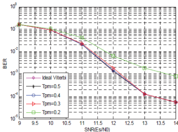
Figure 3. BER performance of T-algorithm
