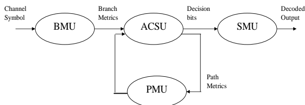
Figure 1. Functional diagram of a Viterbi Decoder
