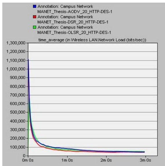
Fig 1: Network Load comparison in three routing protocols for 20 nodes
