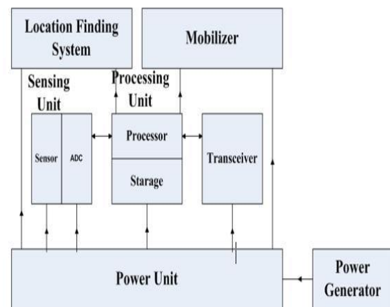
Fig.1 Basic Architecture of Wireless Sensor Network
