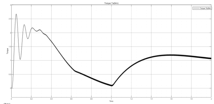
Fig. torque vs. Time of a 3 phase IM speed control induction motor for PI control for V/f control method
