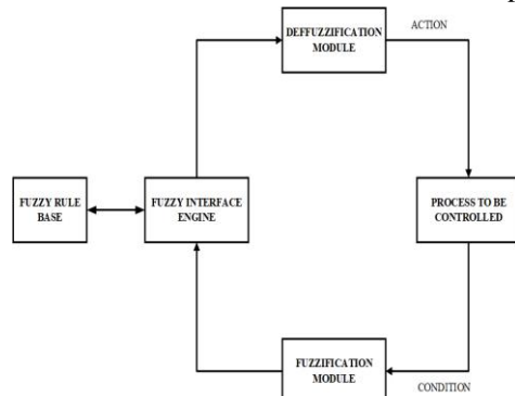
Fig. Block Diagram of Mamdani approach of FLC
