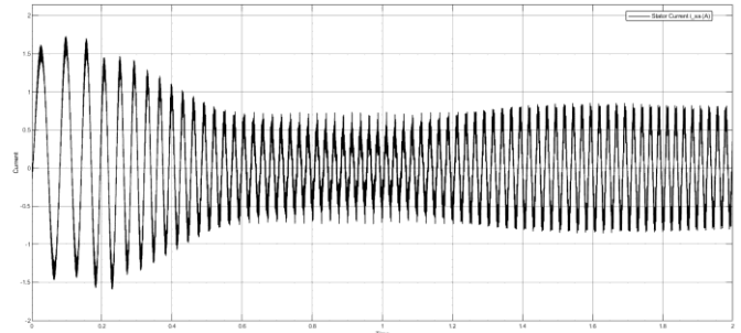
Fig. Stator current of a 3 phase IM speed control induction motor for PI control for V/f control method
