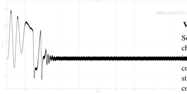
Fig, Torque vs time plot using Fuzzy controller
