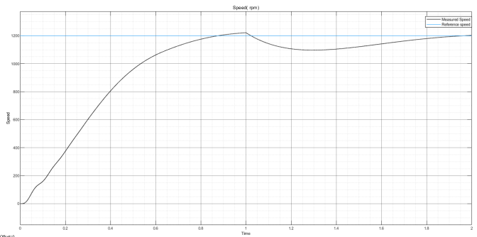
Fig. Speed vs. Time of a 3 phase IM speed control induction motor for PI control for V/f control method
