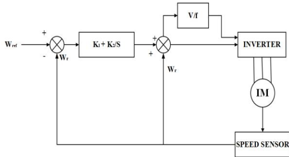
Fig V/f & PI controller block diagram
