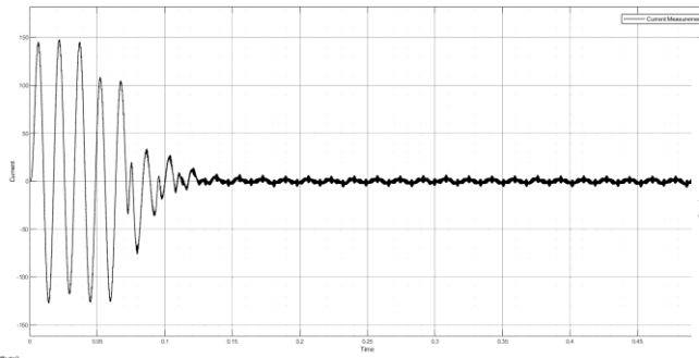
Fig, Stator Current vs time plot using Fuzzy controller
