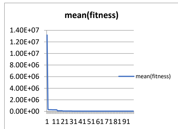
Fig. 5 Convergence of mean value of fitness function over iteration count
