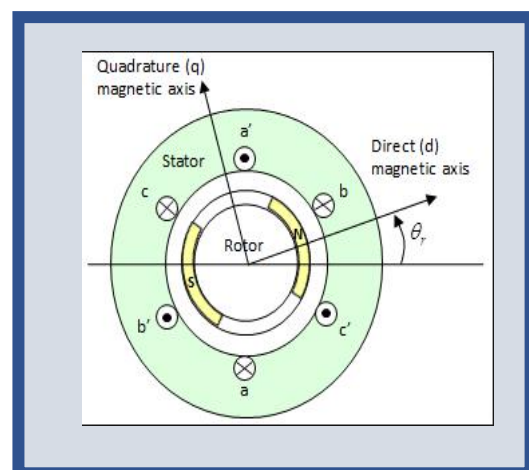
Fig. 1 Cross-sectional view of the motor
