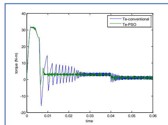
Fig. 7 Response of torque concerning the time
