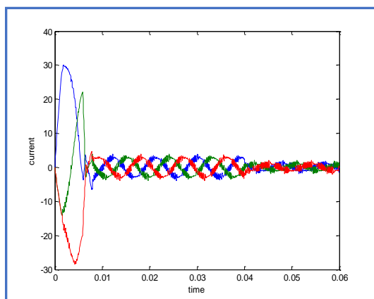
Fig. 8 response of three-phase current of PSO optimize PMSM motor.
