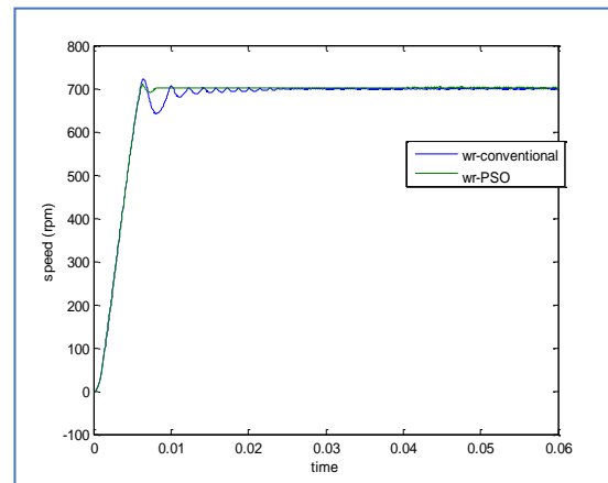
Fig.6 Comparative response of speed of PMSM motor concerning the time
