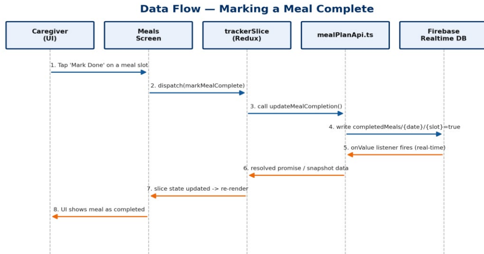
Fig. 2. Sequence diagram for marking a meal complete, showing the eight-step round trip from UI tap to synchronised state.
