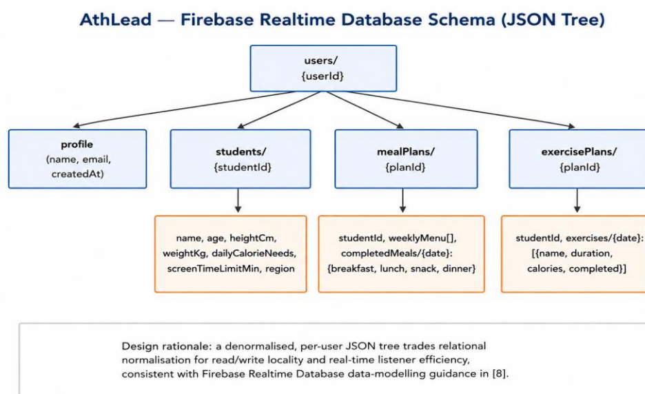
Fig. 3. Firebase Realtime Database schema for AthLead, rooted at users/{userId} .
