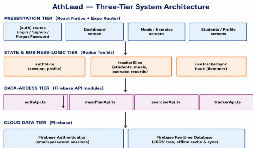
Fig. 1. AthLead three-tier system architecture: presentation, state/business-logic, data-access, and cloud data tiers.
